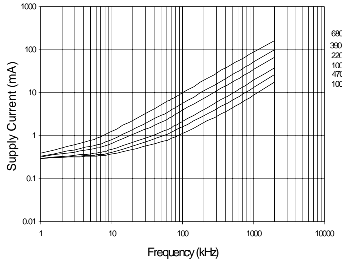
Fig. 12 Supply Current vs. Frequency V CC = 12V
