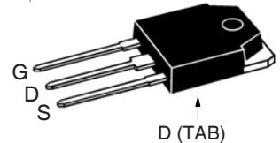
TO-3P (IXFQ)
