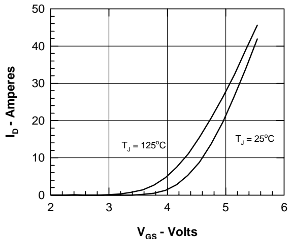
Figure 6. Admittance Curves
