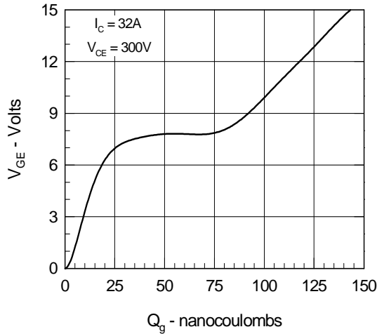
Fig. 9. Gate Charge
