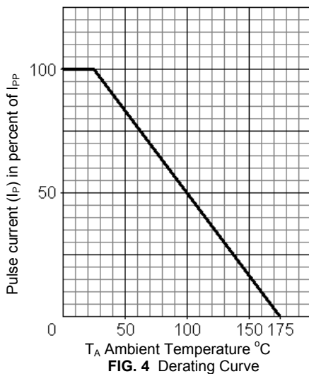
FIG. 4 Derating Curve
