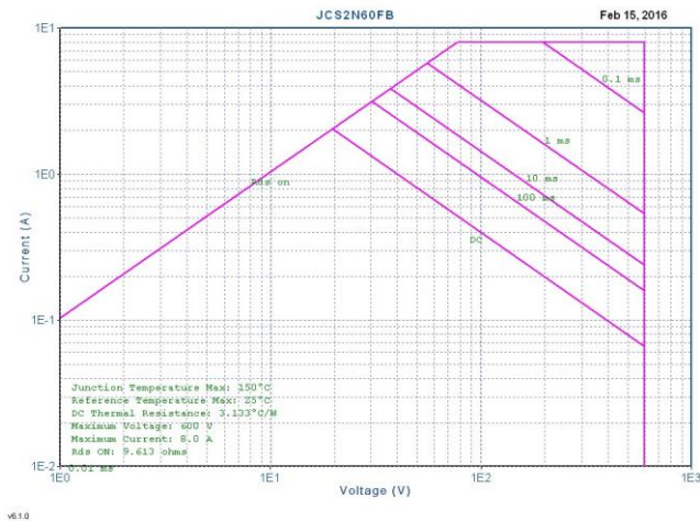
Maximum Safe Operating Area For JCS2N60VB/RB/CB/IB/UB/FB
