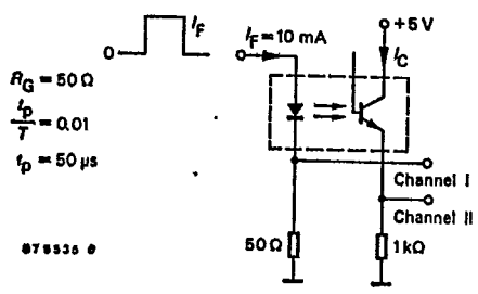
Fig. 2 Test circuit, saturated operation
