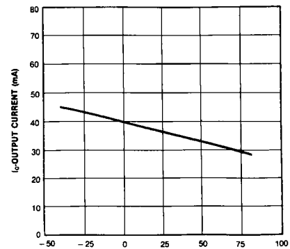
Figure 12. Current Limiting vs Temperature
