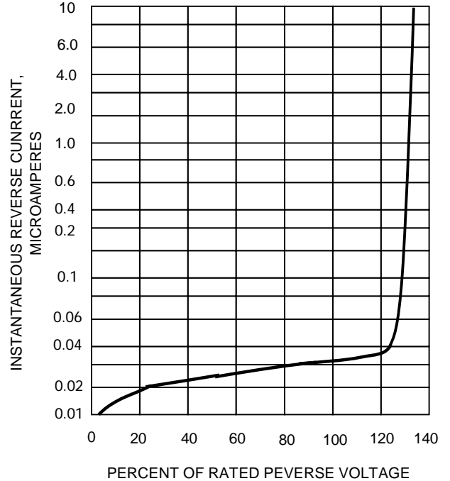
FIG.4-TYPICAL REVERSE CHARACTERISTICS
