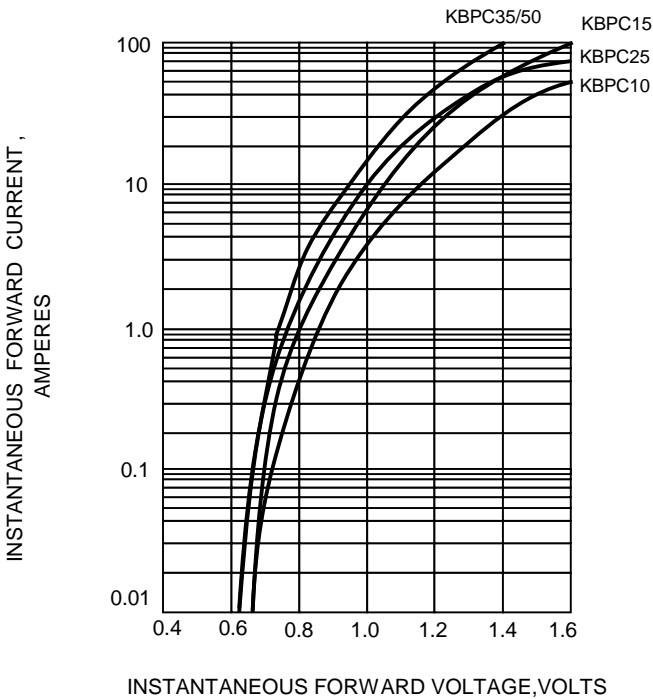
FIG.3-TYPICAL FORWARD CHARACTERISTICS
