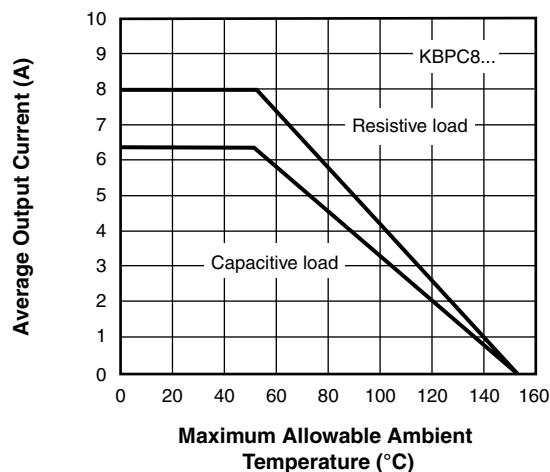
Fig. 1 - Current Ratings
