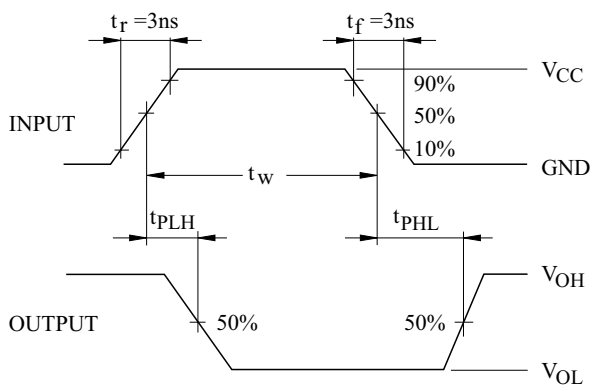
FIGURE 3. AC Waveforms
