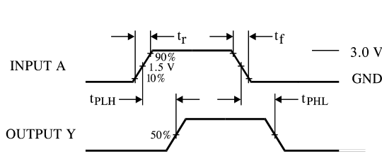
Figure 1. Switching Waveforms
