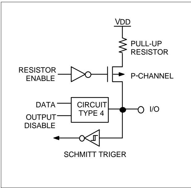
Figure 1-7. Pin Circuit Type D-1
