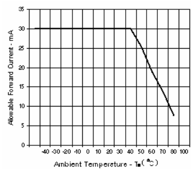
Figure 5-b: Maximum Allowable Forward Current vs. Ambient Temperature – Blue and Green
