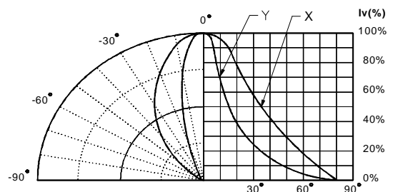
Figure 1-b: Spatial Radiation Pattern - 70°/30°
