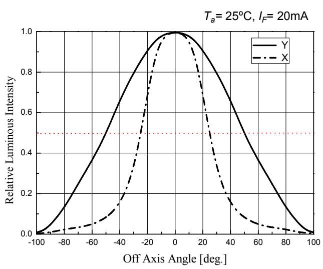
Directivity
