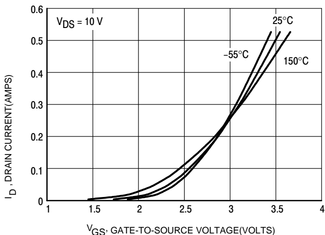
Figure 1. Transfer Characteristics
