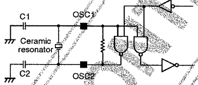
Figure 3. Ceramic resonator option
