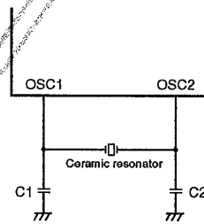
Figure 6. Ceramic resonator
