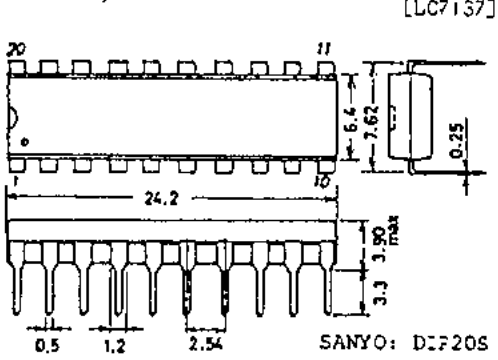
Case Outline 3008A-D20IC (unit:mm)
