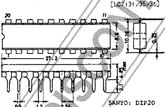
Case Outline 3021B-D20SIC (unit:mm)
