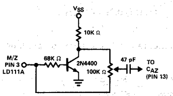
Offset Nulling Circuit Figure 6
