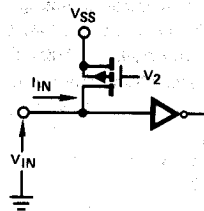
LD110 COMPARATOR, CLOCK INPUTS
