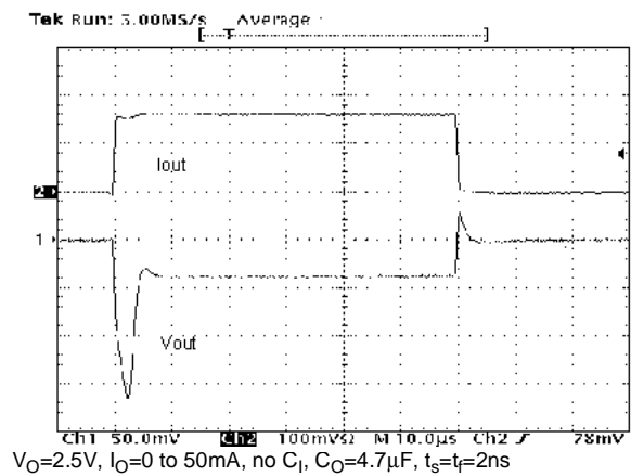
Figure 14 : Load Transient
