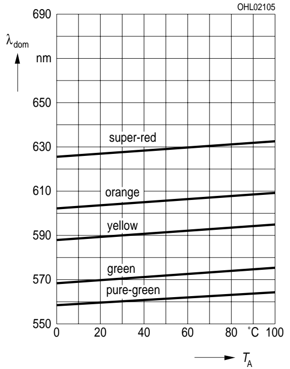
Dominantwellenlänge \lambda_{\text{dom}} = f(T_A) Dominant wavelength I_F = 10 \text{ mA}
