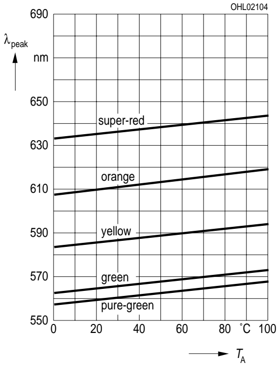
Wellenlänge der Strahlung \lambda_{\text{peak}} = f(T_A) Wavelength at peak emission I_F = 10 \text{ mA}
