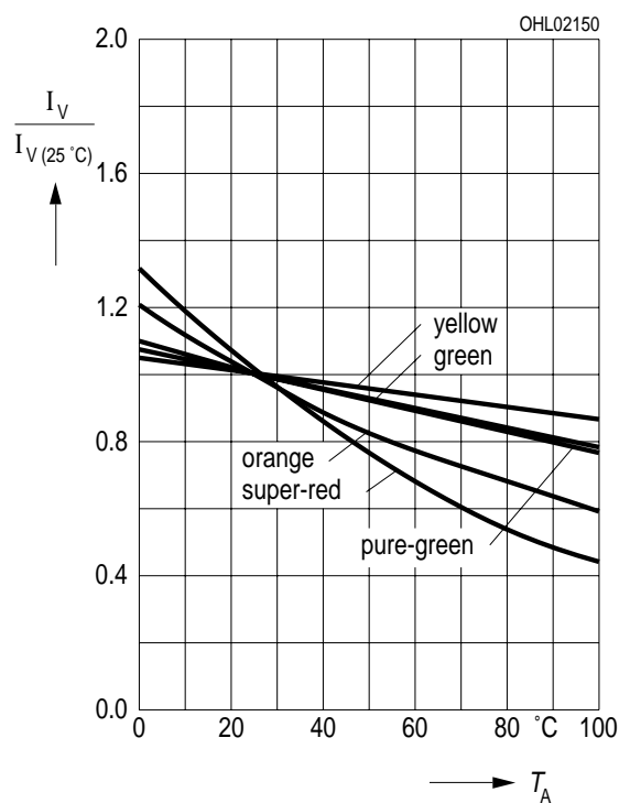
Relative Lichtstärke I_V / I_{V(25^\circ\text{C})} = f(T_A) Relative luminous intensity I_F = 10 \text{ mA}
