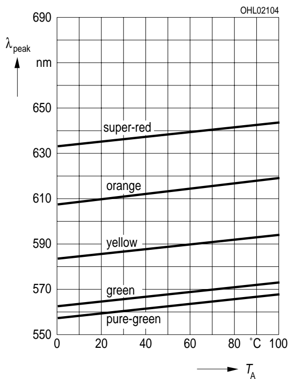
Wellenlänge der Strahlung \lambda_{peak} = f(T_A) Wavelength at peak emission I_F = 20 mA
