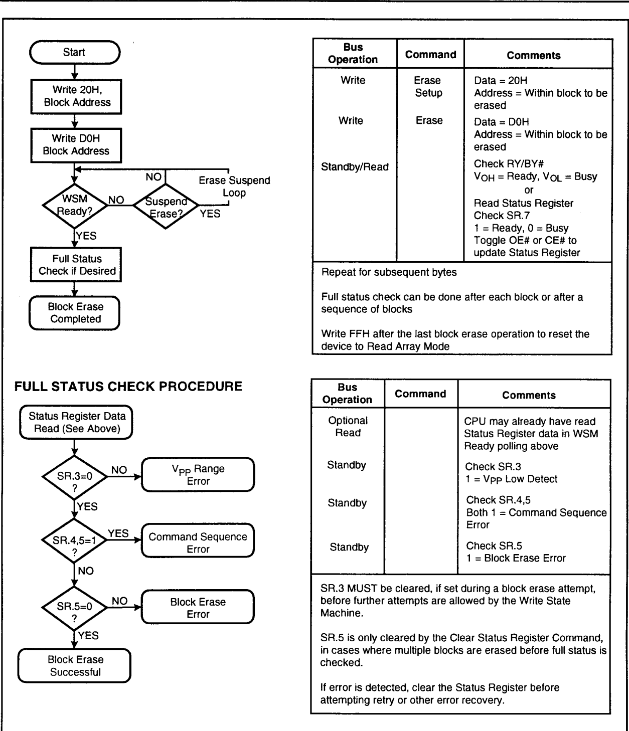
Figure 6. Automated Block Erase Flowchart
