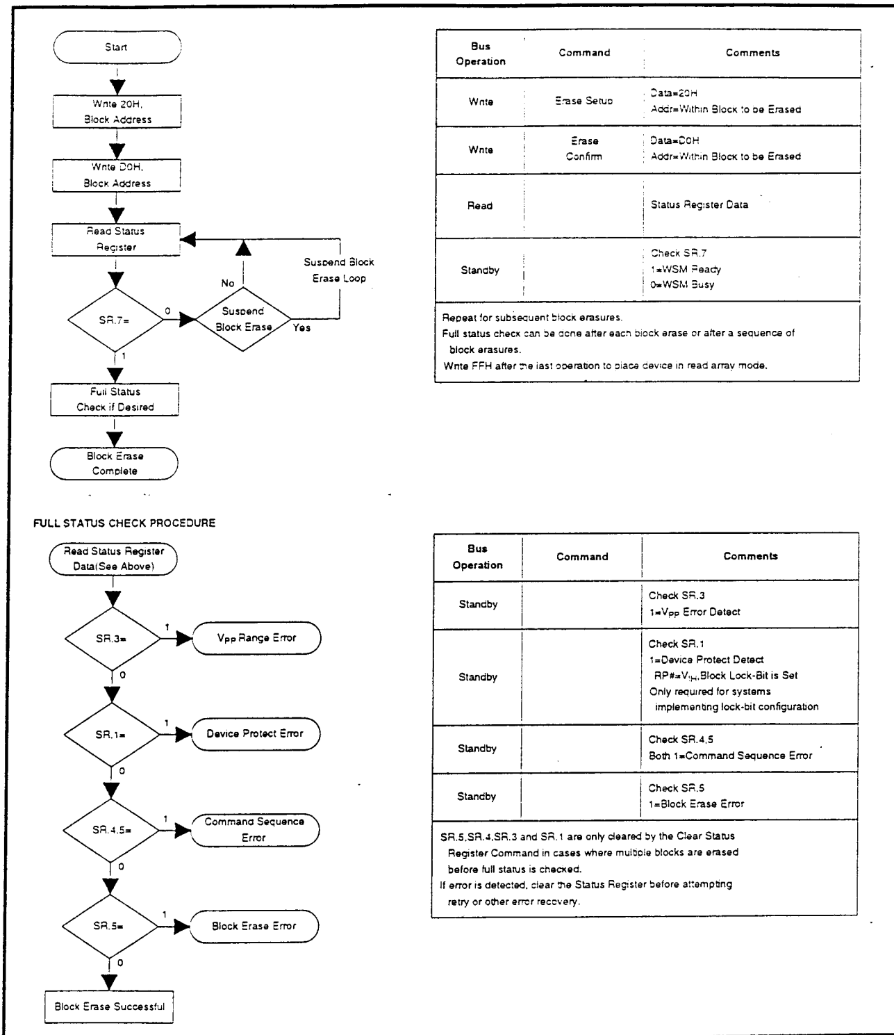
Figure 8. Automated Block Erase Flowchart
