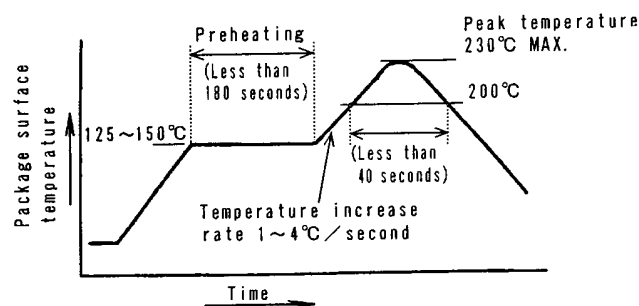
Recommended Reflow Soldering(Air) Temperature Profile
