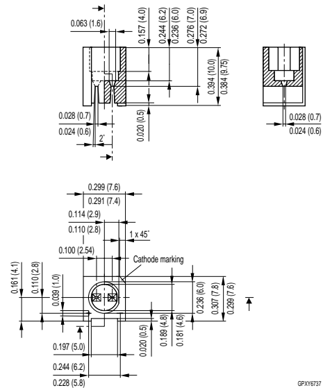
Figure 38 Winkelhalterungen für 5 mm LED Rectangular mounting part for 5 mm LED Q62902-B156-F222 (grey)
