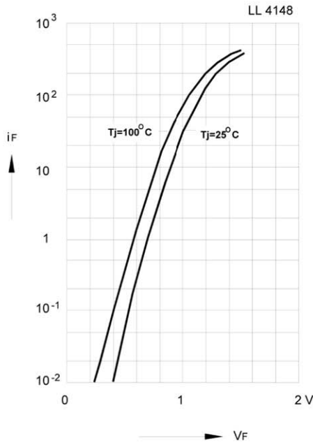
Forward characteristics
