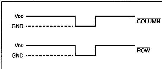
Fig. 4 Electronic Input
