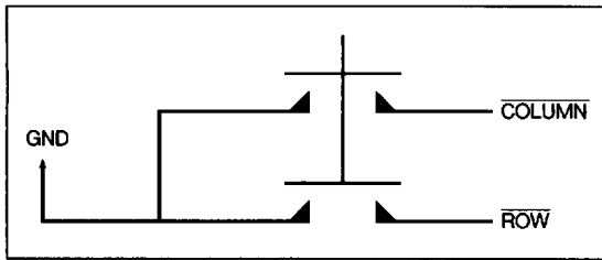
Fig. 3 Keyboard Configuration
