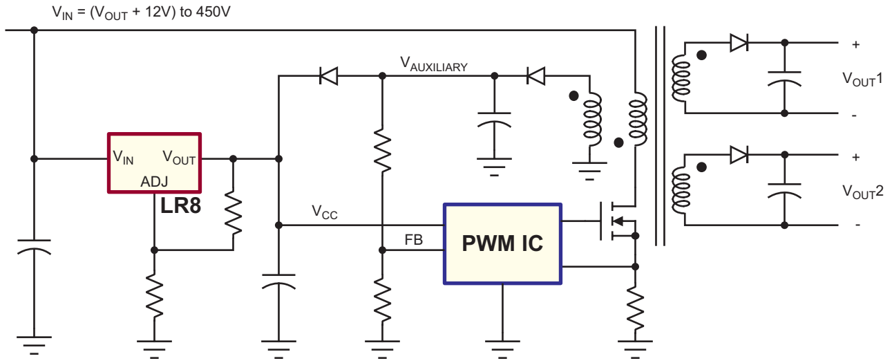
Figure 2: SMPS Start-Up Circuit
