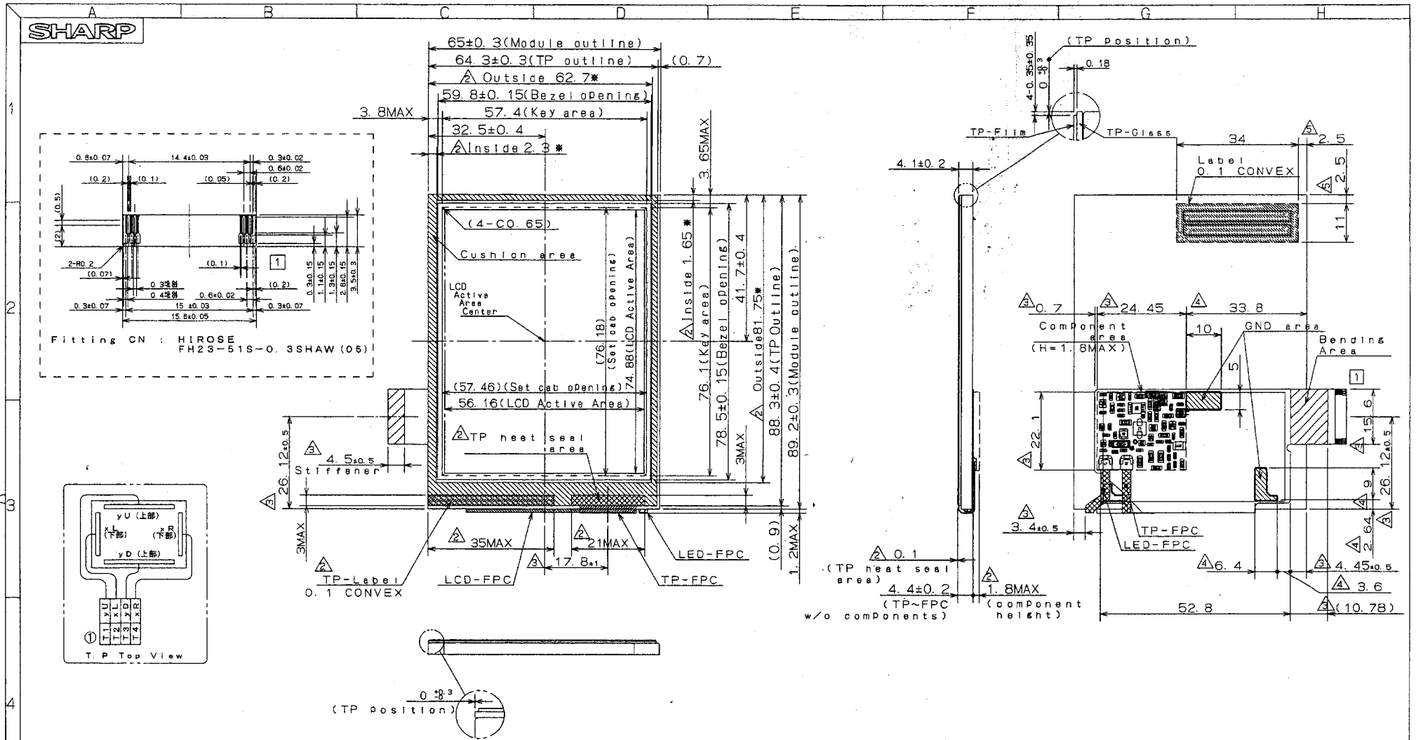
Fig. 1 Outline dimensions
