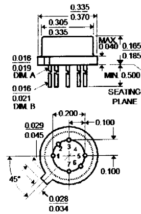
TO-78
