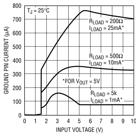
LT1121-5 Ground Pin Current
