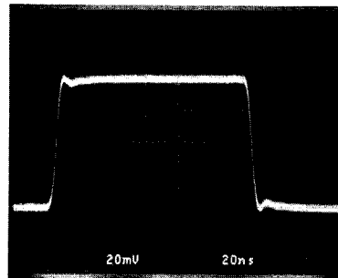
A_V = +2 , WITH 8\text{pF} FEEDBACK CAPACITOR RISE TIME = 3.75\text{ns} , R_{FB} = 1\text{k} , R_G = 1\text{k}
