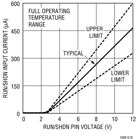
RUN/SHDN Input Current vs Pin Voltage
