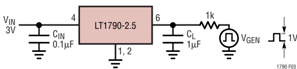
Figure 3. Response Time Test Circuit
