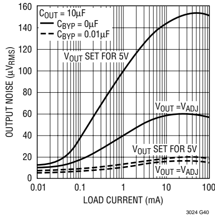
Output 2 RMS Output Noise vs Load Current (10Hz to 100kHz)
