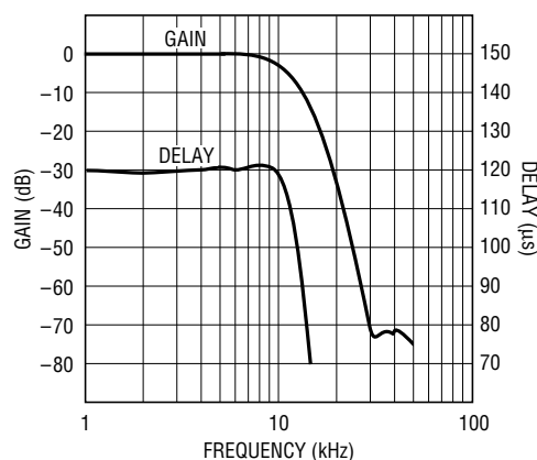
Frequency Response
