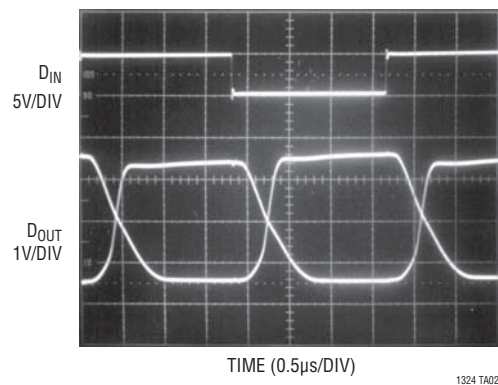
Waveform of Driver
