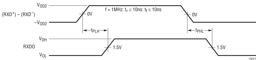
Figure 6. Differential Receiver
