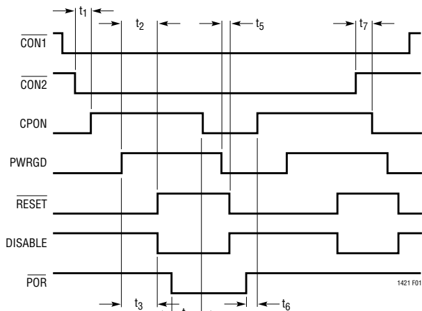
Figure 1. Nominal Operation Switching Waveforms
