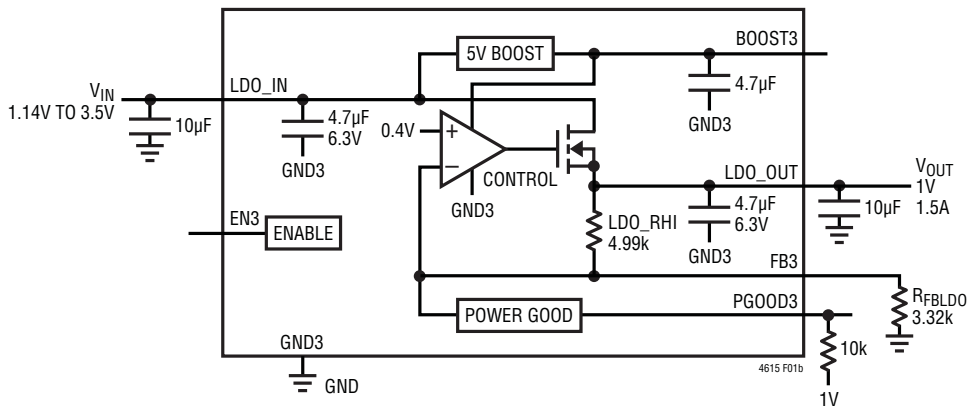
Figure 1. Simplified LTM4615 Block Diagram of Each Switching Regulator Channel and the VLDO
