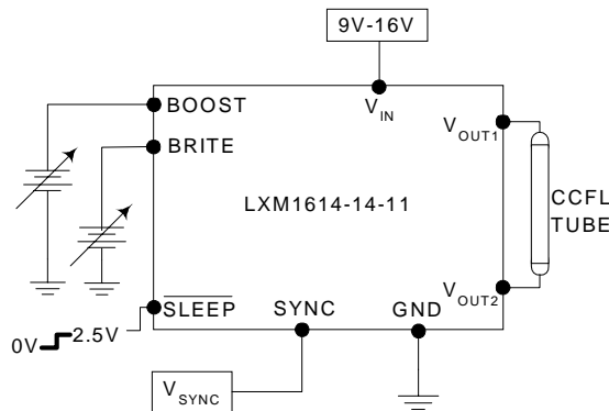
Figure 11 - Brightness Control
