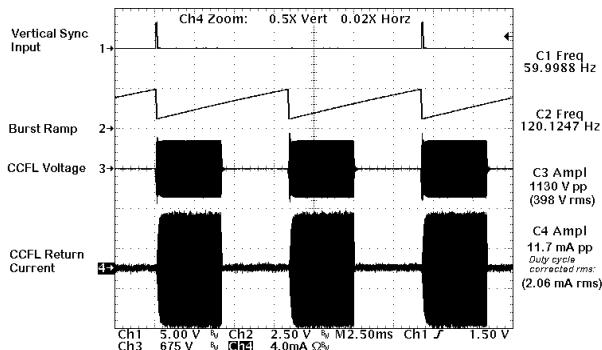
Figure 3 – 50% Burst Duty Cycle
