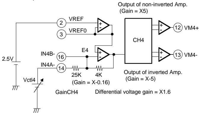
CH4 amplifier
