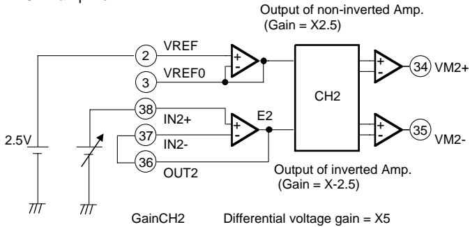
CH2 amplifier
