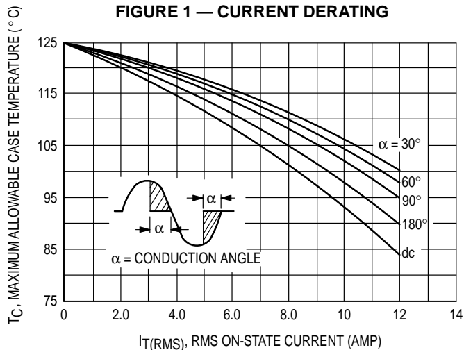
FIGURE 1 — CURRENT DERATING
