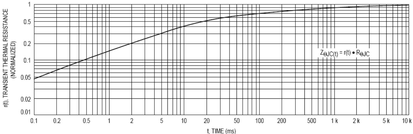
FIGURE 8 — THERMAL RESPONSE
