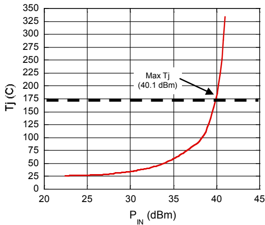
Tx Diode Junction Temperature vs. C.W. Input Power @ 4.0 GHz, T_j = 175^\circ\text{C}
