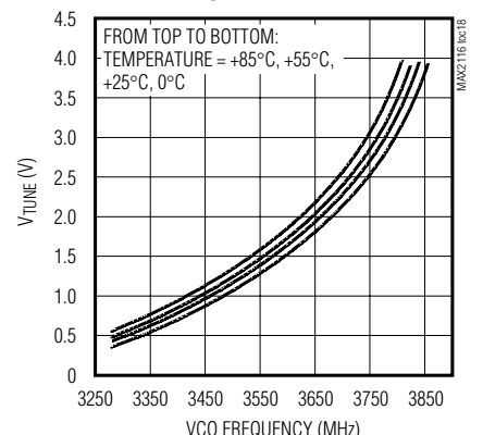
VCO_4: V TUNE vs. VCO FREQUENCY
