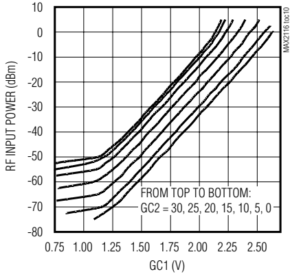
RF INPUT POWER vs. GC1 (BASEBAND OUTPUT = 800mV _{P-P} )
