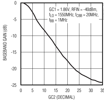
BASEBAND GAIN vs. GC2
