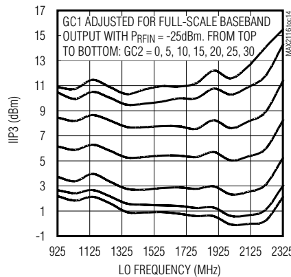
IIP3 vs. LO FREQUENCY
