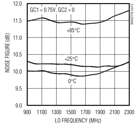
NOISE FIGURE vs. LO FREQUENCY
