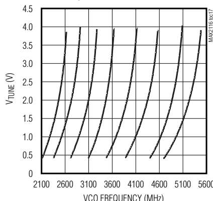
V TUNE vs. VCO FREQUENCY
