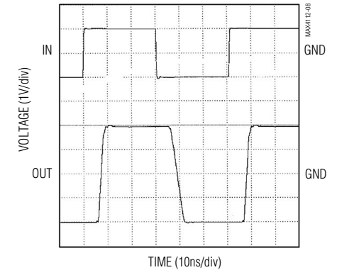
MAX4112/MAX4117/MAX4119 LARGE-SIGNAL PULSE RESPONSE ( A_{VCL} = +2 )
