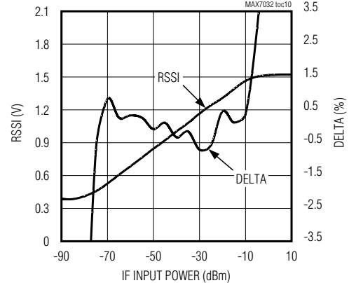
RSSI AND DELTA vs. IF INPUT POWER
