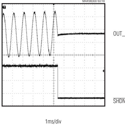
STARTUP WAVEFORM
